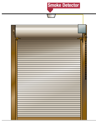
FD-2A Auto-Test Chain Operated Fire Door System
