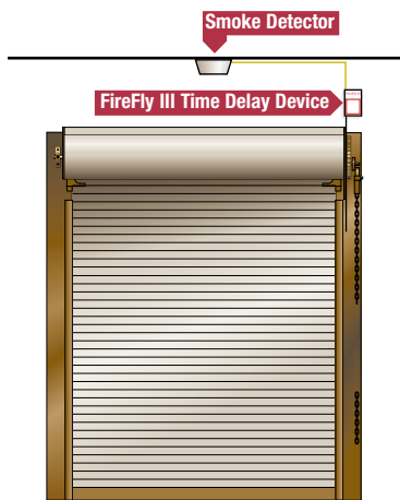
Simple-Test Fire Door System with FireFly III
