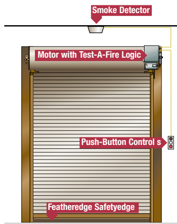
FDO-A Auto-Test Motor Operated Fire Door System
